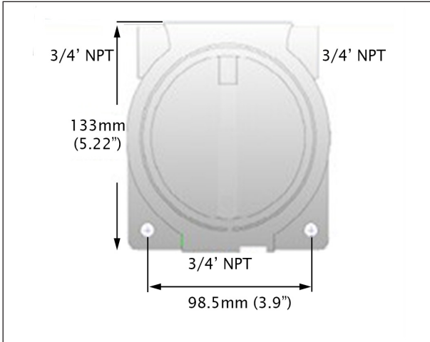
Figure 1: Mounting details
